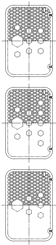
鉄蓋角型6号A (1200X770)
