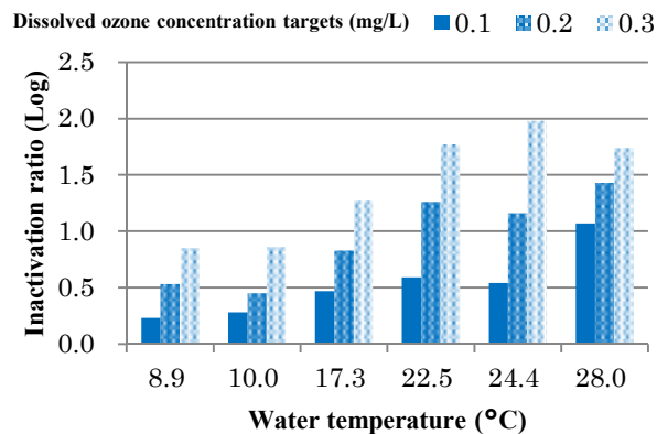
Figure 8: Inactivation ratios in ozone treatment
