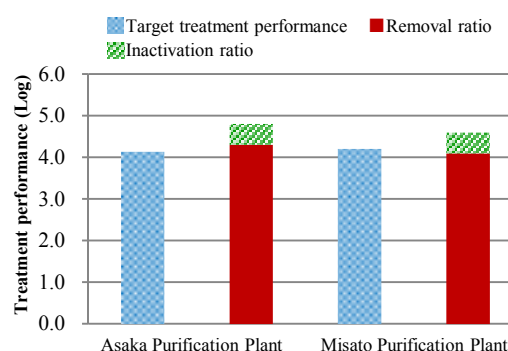
Figure 12: Target treatment performance values and removal-inactivation ratios
