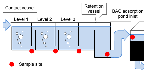
Figure 3: Ozone treatment and BAC adsorption pond
