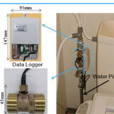
Figure 3. Flow Sensor and Data Logger
