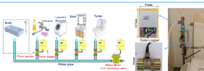
Figure 2. Measuring and recording water consumption
