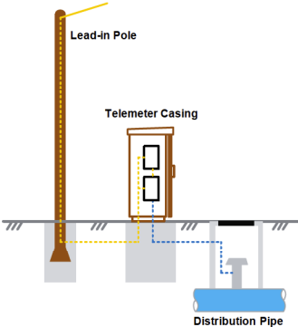
Figure 2 - Layout of Aboveground Telemeter
