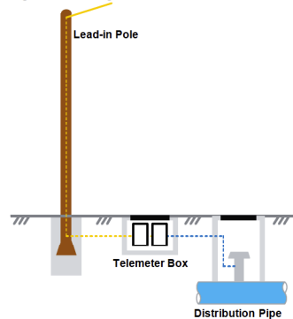
Figure 4 - Layout of Underground Telemeter
