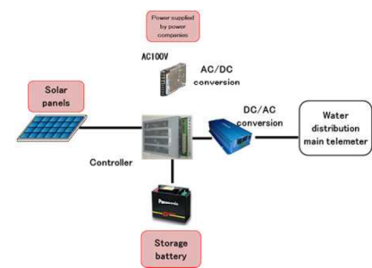
Figure 3: Chart of the three-power source system configuration
