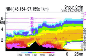
Figure 8. Typical example of number concentration of AgI particles released from ground-based generators
