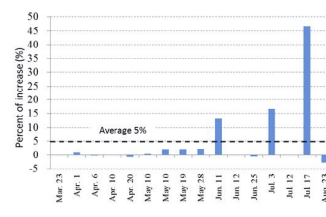
Figure 7. Effects of ground-based AgI seeding on rainfall over the Ogouchi Reservoir drainage area
