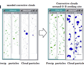
Figure 6. Comparison of ice crystals
