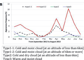
Figure 5. Occurrence frequency of seedable clouds
