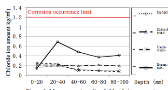
Figure 3: Measurement results of chloride ion amount
