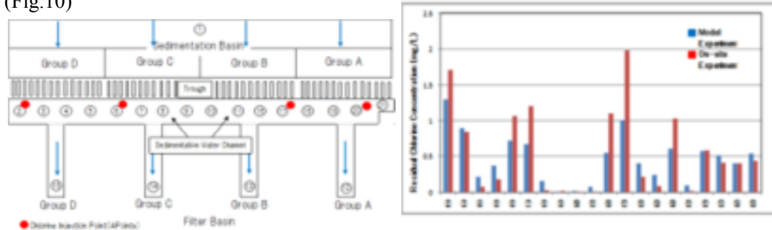
Figure 10 Residual chlorine concentration in actual facility and model with "Method A"
