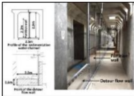
Figure 16 Partition wall and detour flow wall installed Figure 17 Partition wall installed in sedimentation water channel
