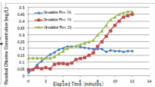
Figure 14 Circulation flow and time for residual chlorine to reach Group D filter basin
