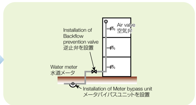
Figure: Piping Example when Changing Water Supply Facilities with Receiving Tanks in Building of Three Stories or Less to Direct Water Service System 3階までの受水タンク以下装置を直圧直結給水方式に切り替える場合の配管例
