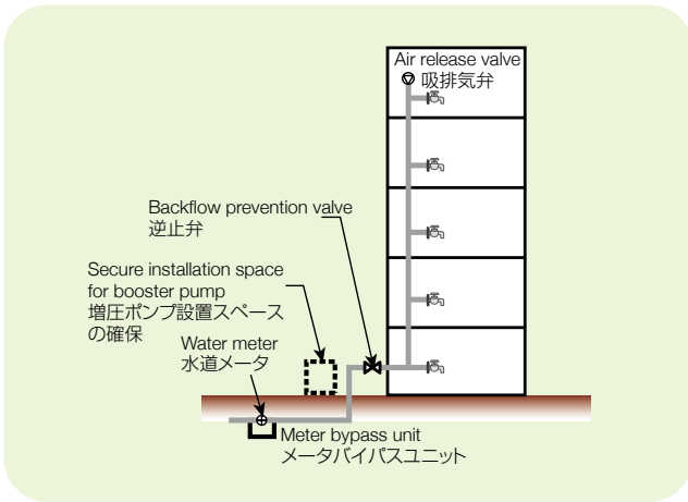
Figure: Exceptional Direct Water Service System 特例直圧直結給水方式
