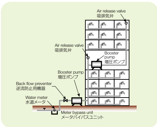
Figure: Pressure Water Service System (series type) 増圧直結給水方式（直列多段型）
