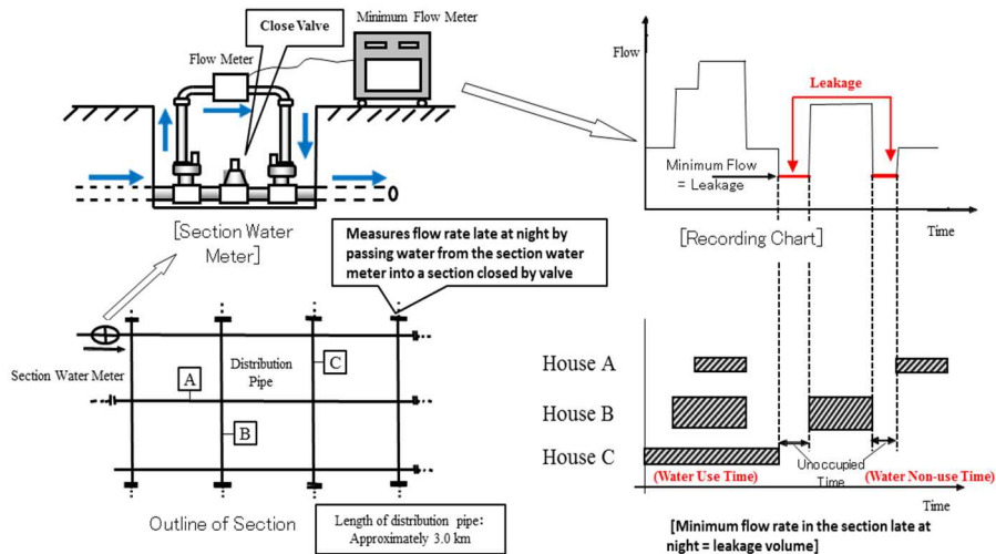
Figure 5 Night Minimum Flow Rate Measurement Method
