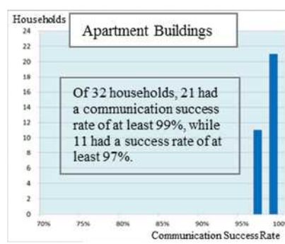
Figure 11. Communication Success Rate Distribution (Apartment Buildings)
