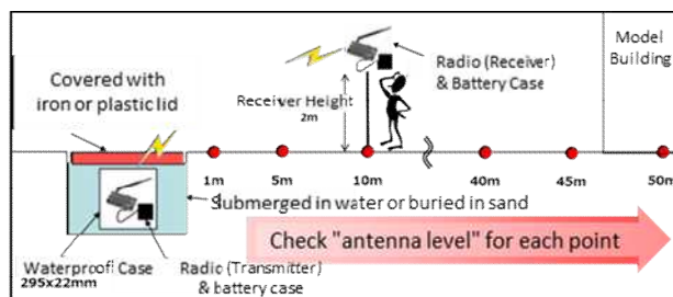
Figure 3. Overview of communication distance measurement
