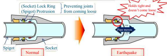
joint of earthquake-resistant joint Pipes (conceptual diagram)
